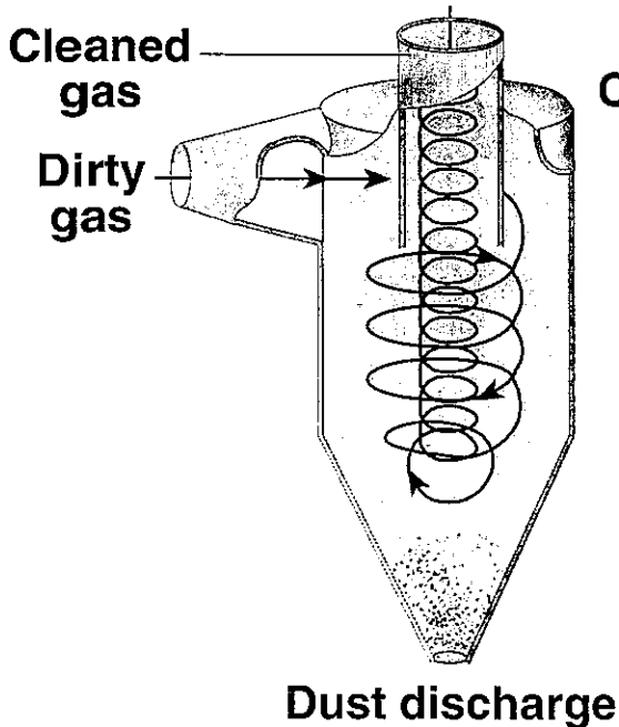
c. Cyclone Separator
